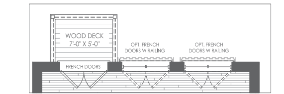
OPTIONAL DECK CONDITION - FOR INTERNAL LOTS ONLY
