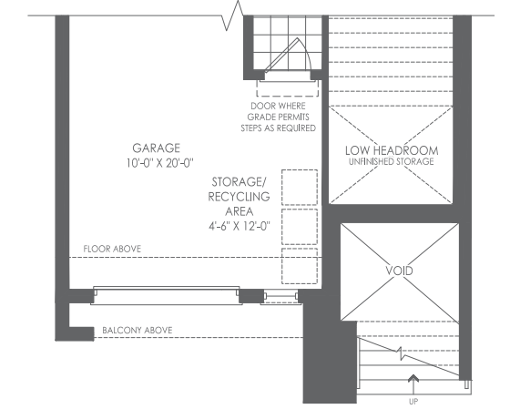
PARTIAL GROUND FLOOR ELEV. B
