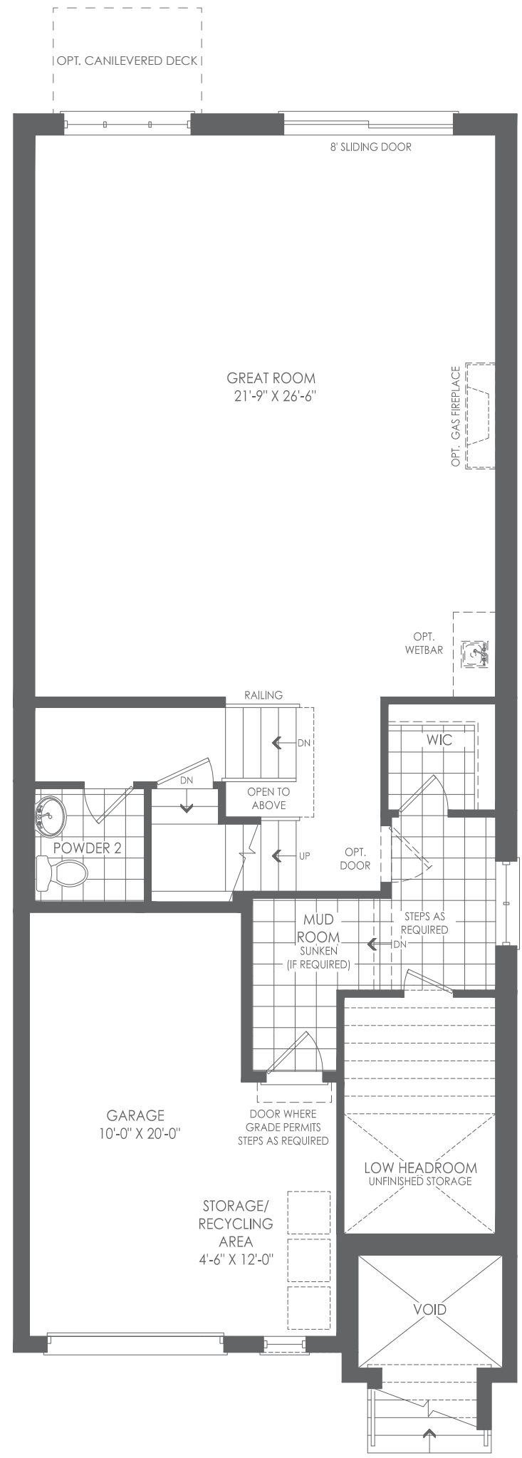
GROUND FLOOR ELEV. A
