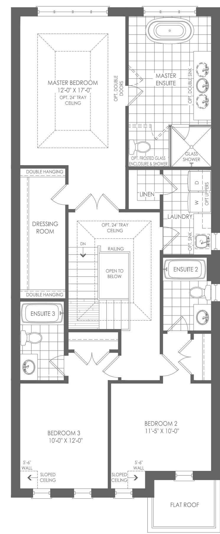
THIRD FLOOR ELEV. A
