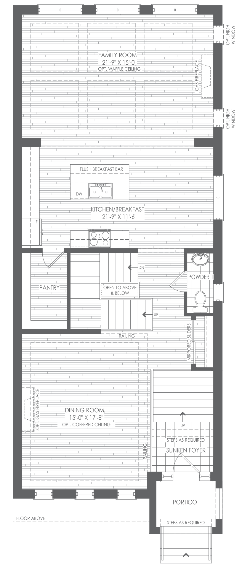
SECOND FLOOR ELEV. A (MAIN LIVING/KITCHEN LEVEL)
