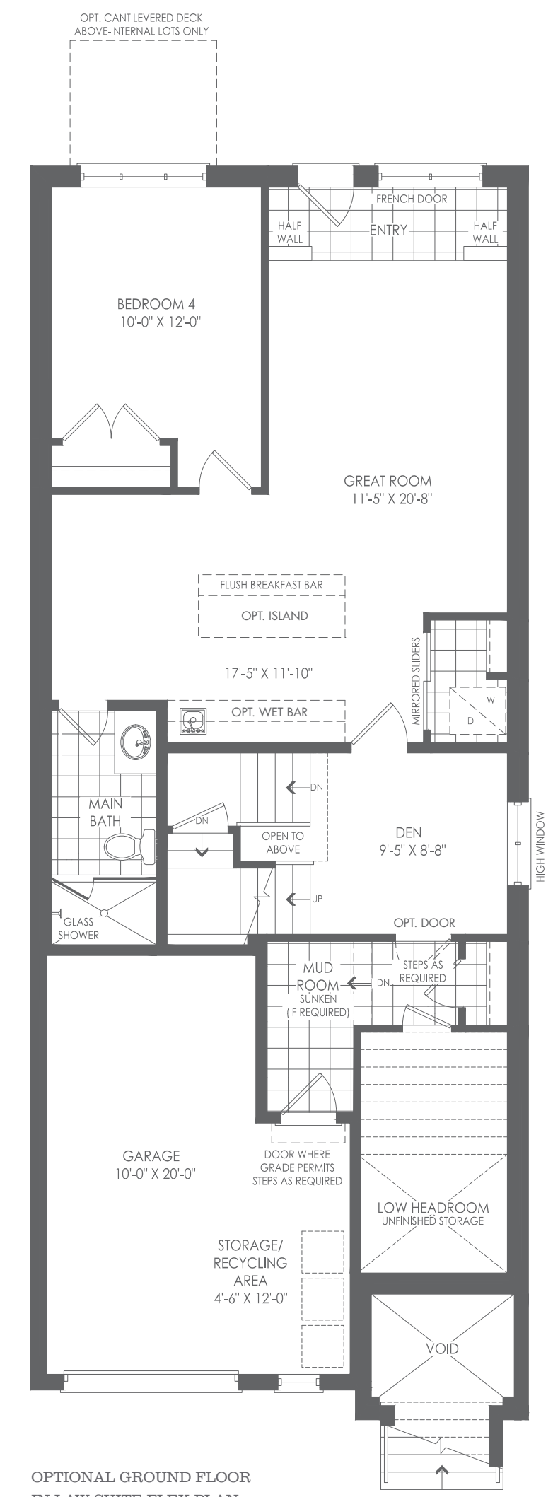
OPTIONAL GROUND FLOOR IN-LAW SUITE FLEX PLAN
